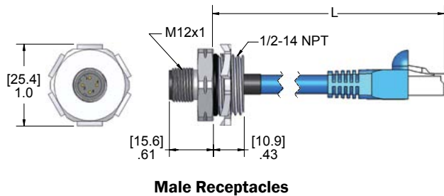
Male Receptacles
