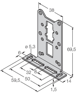
Mounting bracket for rectangular Q14 or Q20; material VA 1.4301
