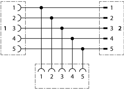
Circuit Diagram
