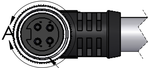
7/8-16UN2B FEMALE THREAD
