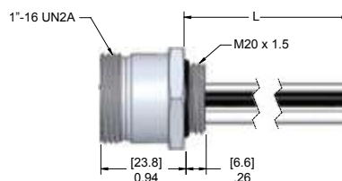
M20 Threads
