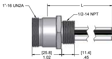
1/2"-14 NPT Threads
