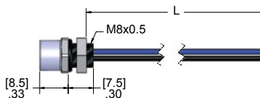
Female Receptacle
