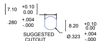
Male Receptacle
