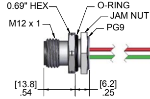
Male Receptacle
