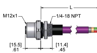
Female Receptacle
