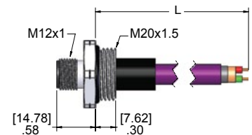
Male Receptacle
