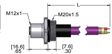
Female Receptacle
