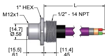
Female Receptacle
