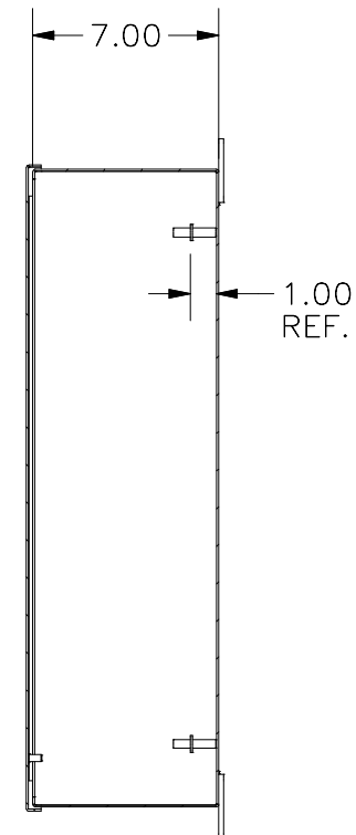
SECTION B-B SIDE VIEW
