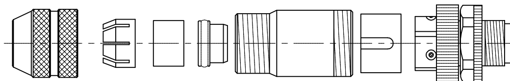
EXPLODED VIEW
