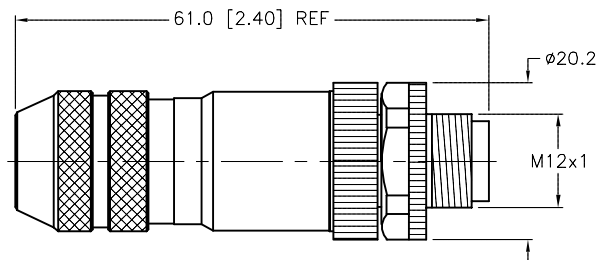
ASSEMBLED VIEW
