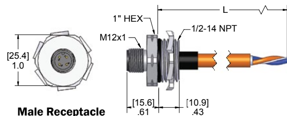
Male Receptacle
