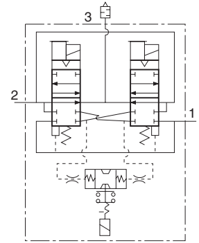
Valve Schematic
