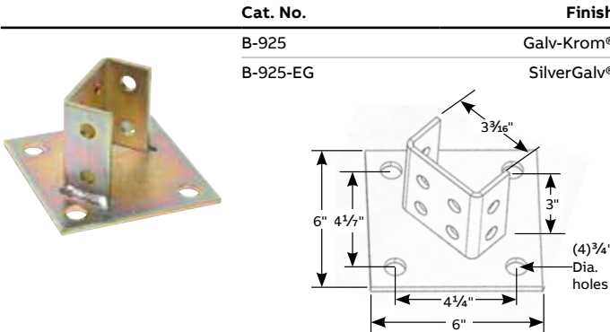
B-925 Post base connector
