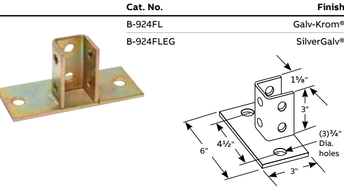
B-924FL Post base connector
