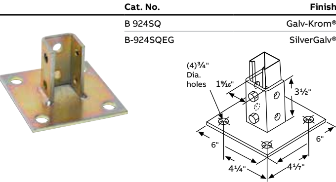
B-924SQ Post base connector
