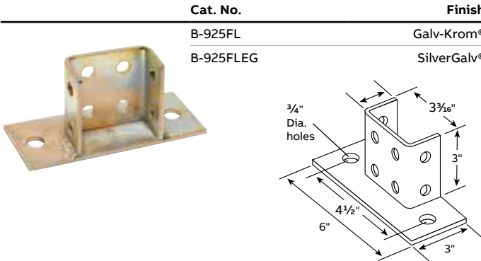
B-925FL Post base connector
