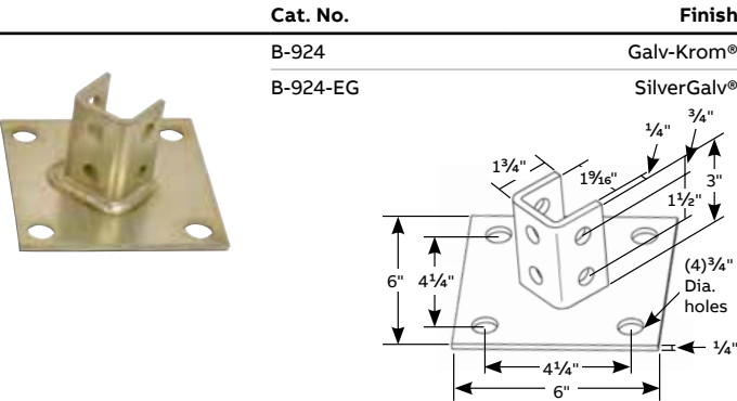
B-924 Post base connector
