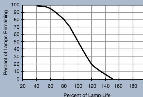
Typical Mortality Curve for Incandescent Lamps
