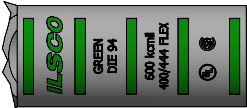
DETAIL B TOP AND BOTTOM INK MARKINGS ARE IDENTICAL INK COLOR:GREEN PER SPEC #: F921
