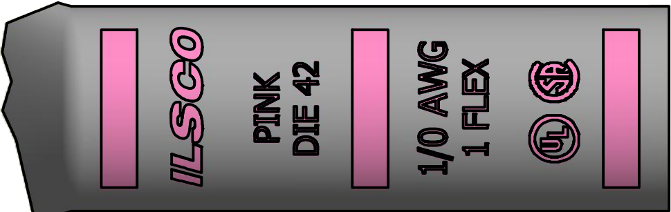
DETAIL C TOP INK MARKING INK COLOR: PINK PER SPEC #: F921
